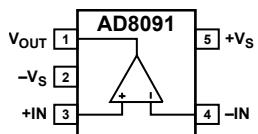
Figure 2. SOT23-5 (RJ-5)
