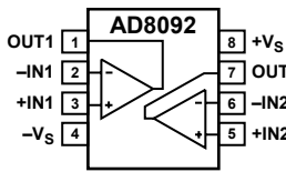
Figure 3. MSOP-8 and SOIC-8 (RM-8, R-8)
